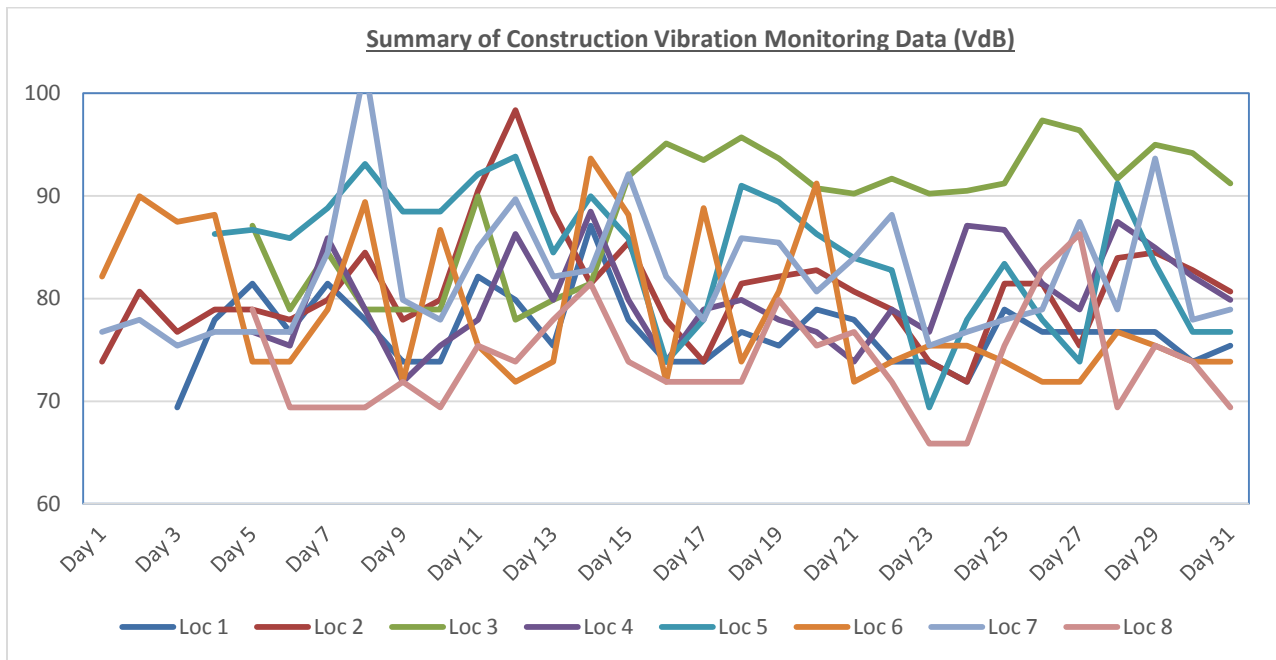
Figure 2. Summary of Construction Vibration Monitoring Data (VdB) – January 2016
