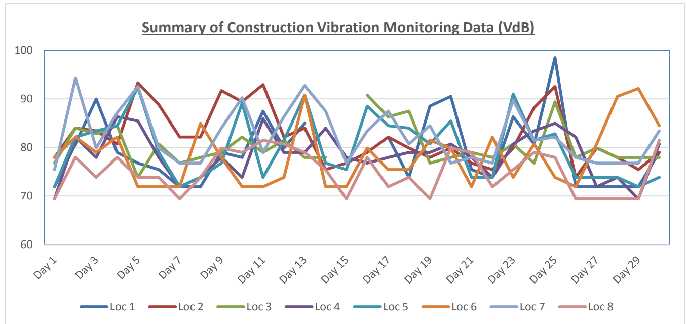
Figure 2. Summary of Construction Vibration Monitoring Data (VdB) – November 2015
