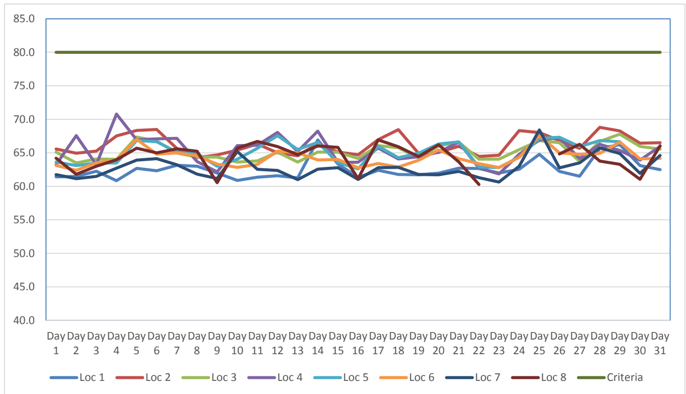
Figure 2. Summary of Daily Construction Noise Monitoring Data dB(A) – July 2017
