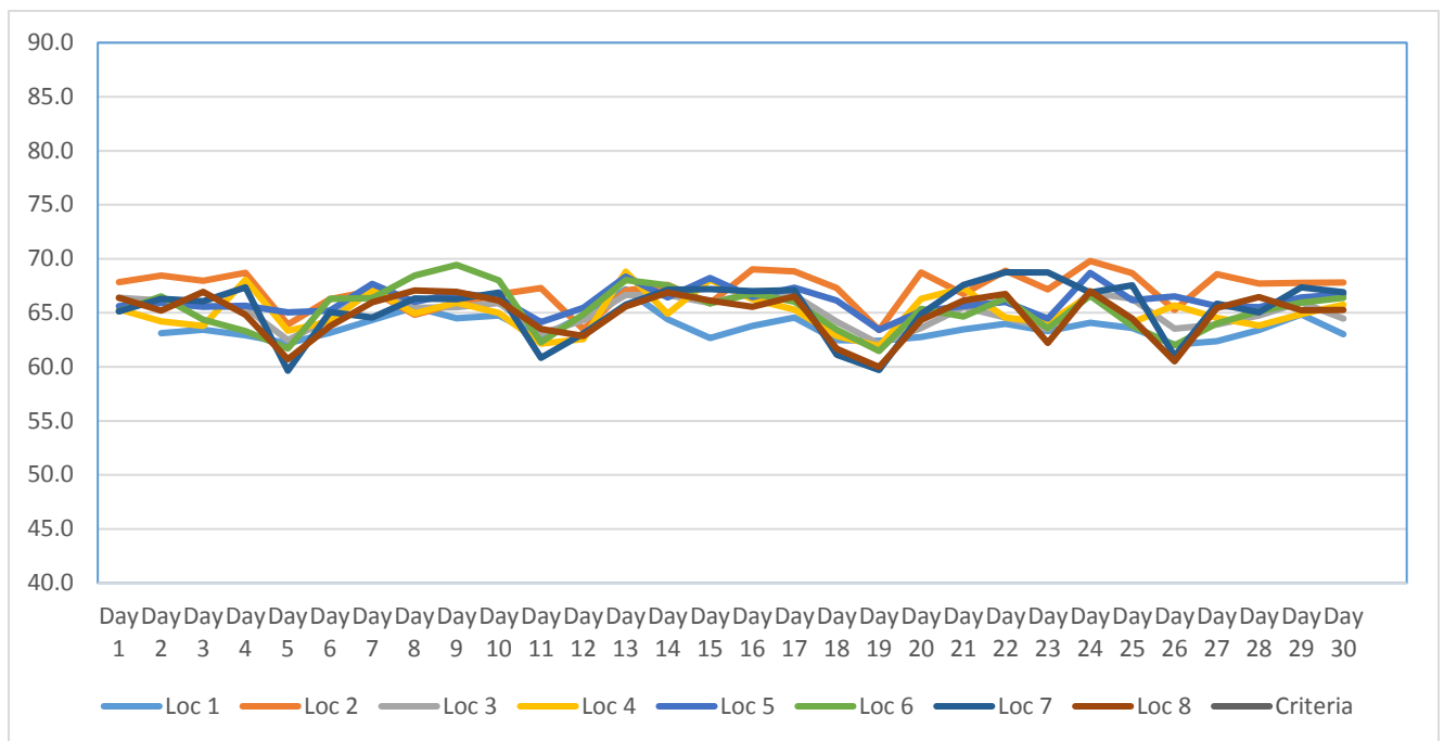
Figure 2. Summary of Daily Construction Noise Monitoring Data dB(A) – June 2016
