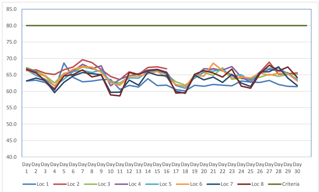
Figure 2. Summary of Daily Construction Noise Monitoring Data dB(A) – June 2017
