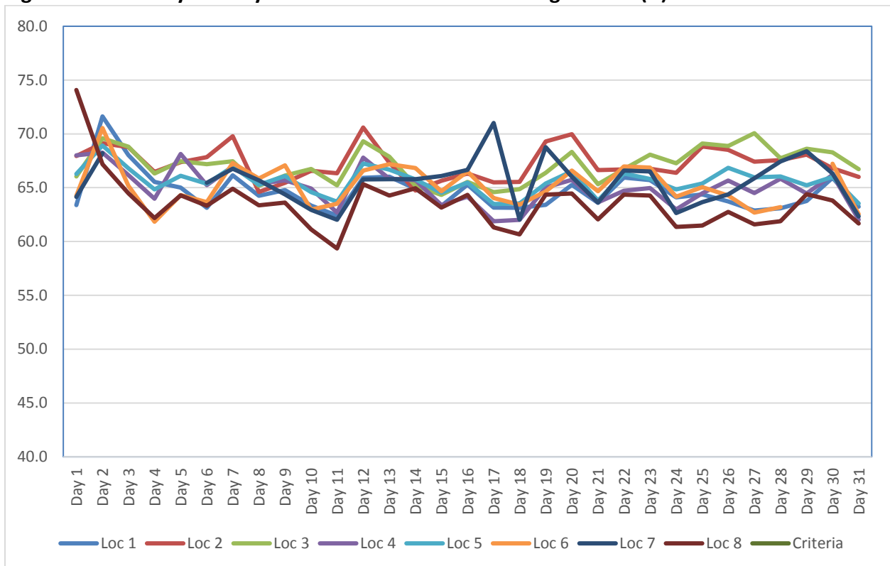
Figure 2. Summary of Daily Construction Noise Monitoring Data dB(A) – March 2018
