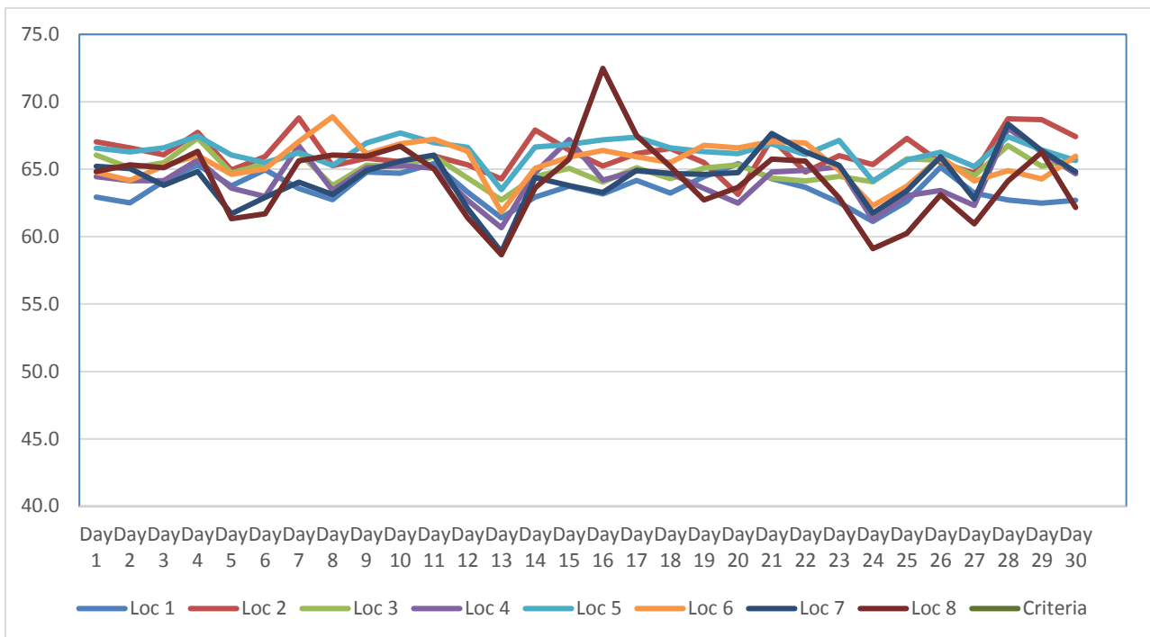
Figure 2. Summary of Daily Construction Noise Monitoring Data dB(A) – November 2016
