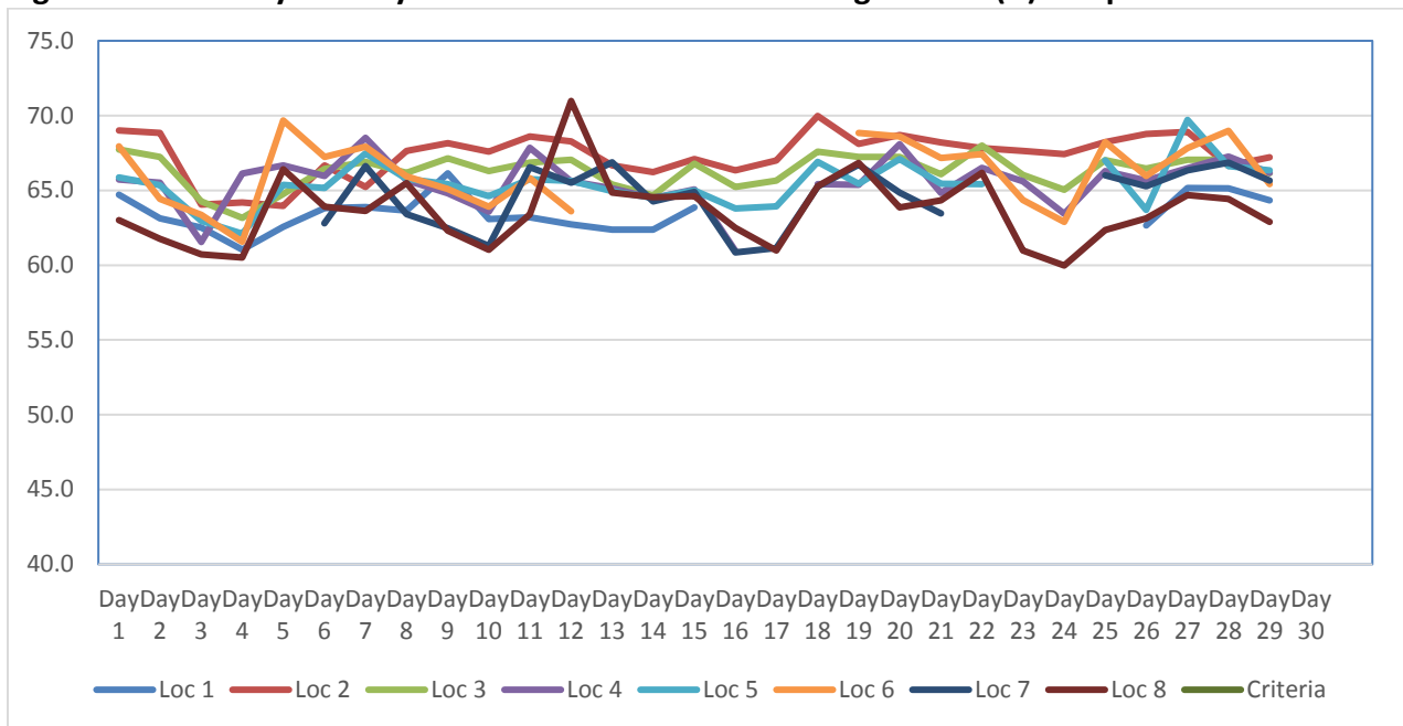
Figure 2. Summary of Daily Construction Noise Monitoring Data dB(A) – September 2017
