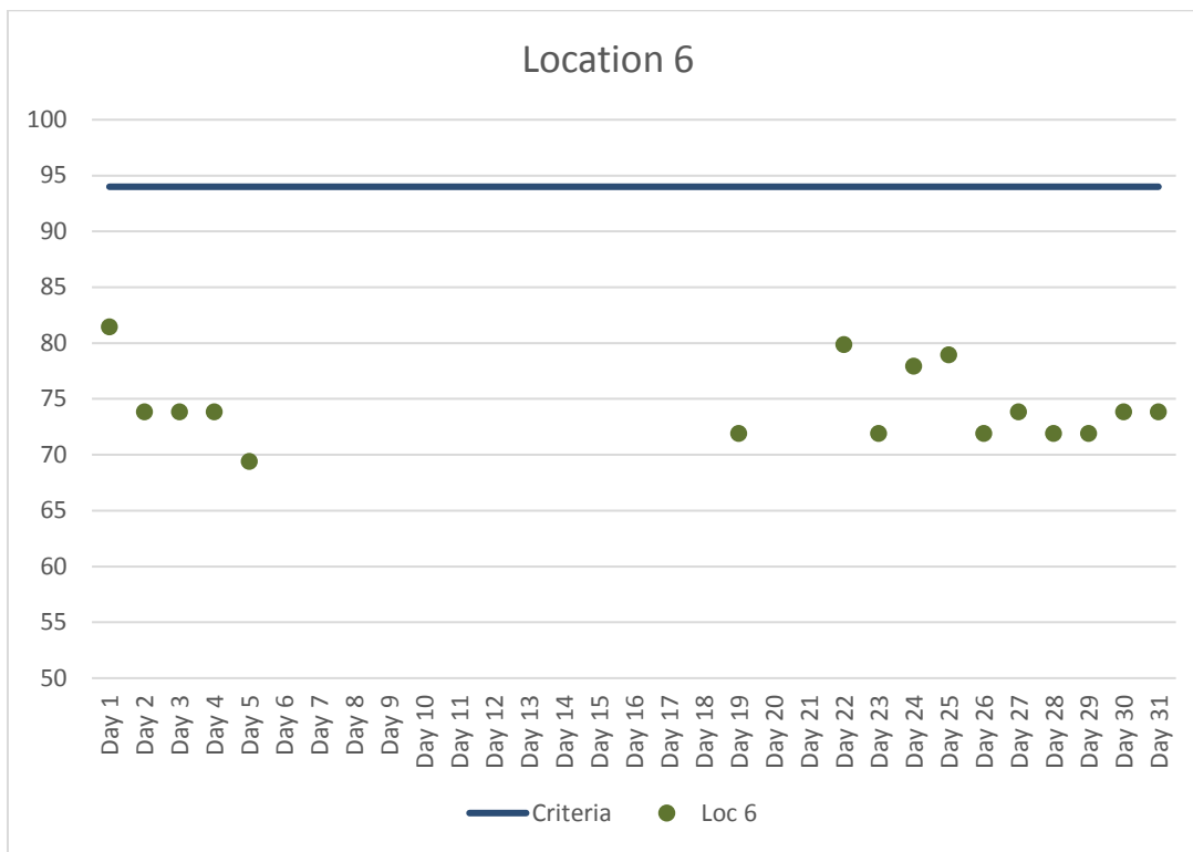
Figure 7. Location 6 Maximum Daily Construction Vibration Monitoring Data (VdB) – May 2017
