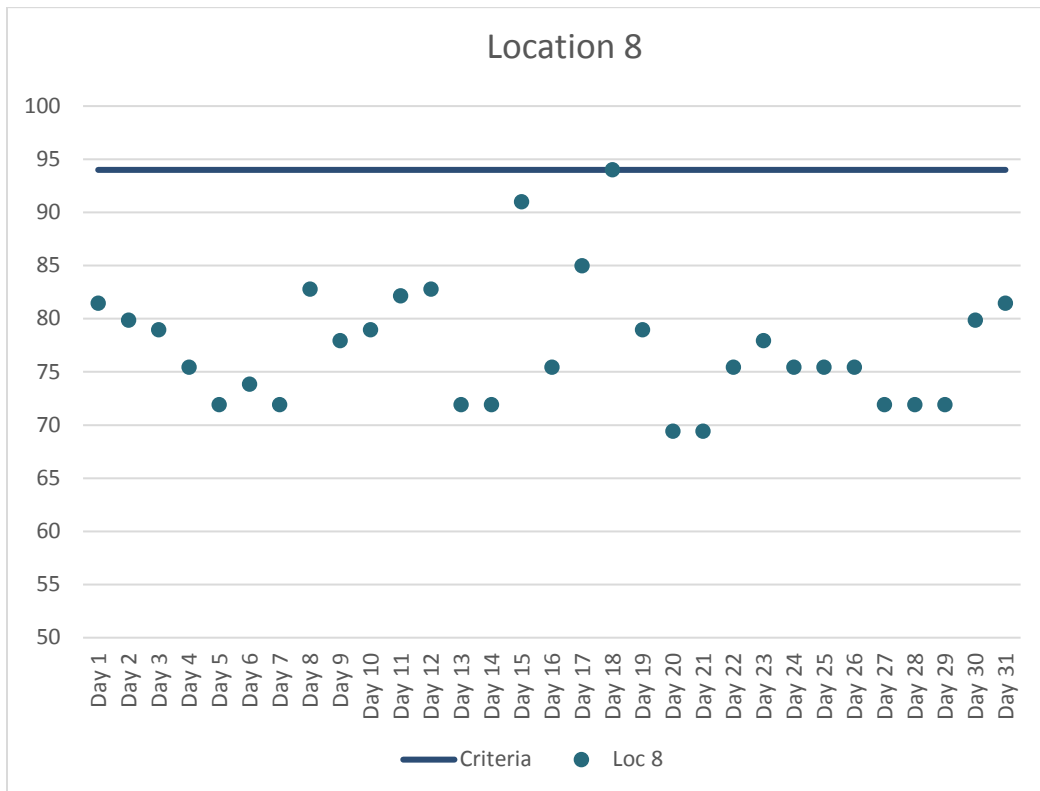
Figure 9. Location 8 Maximum Daily Construction Vibration Monitoring Data (VdB) – May 2017
