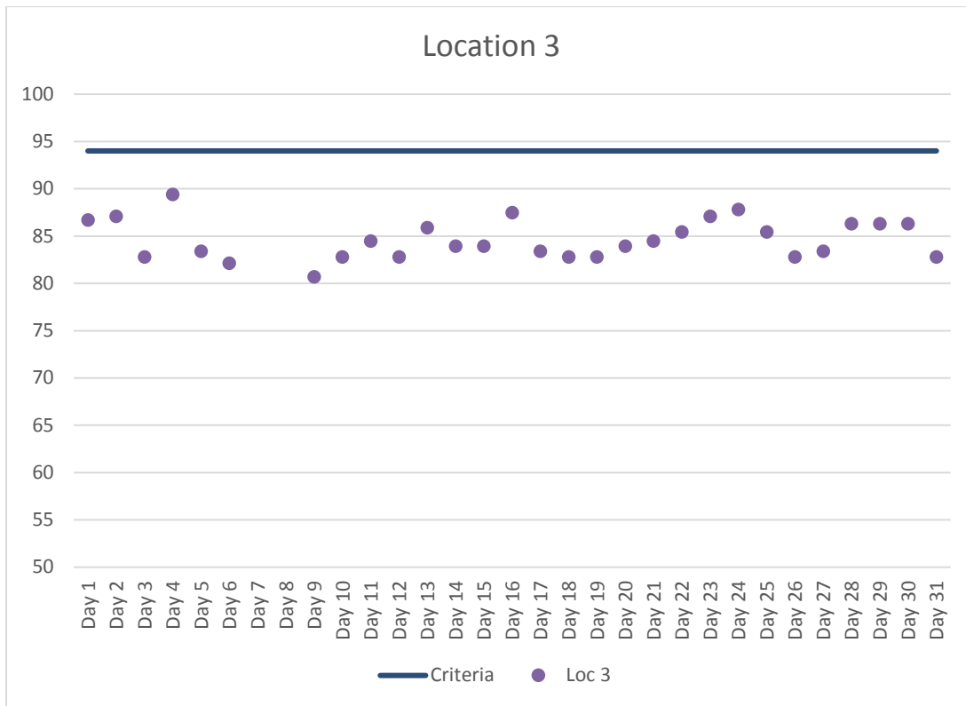
Figure 4. Location 3 Maximum Daily Construction Vibration Monitoring Data (VdB) – May 2017
