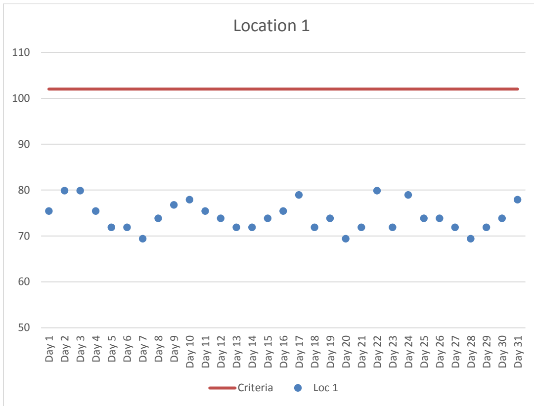
Figure 2. Location 1 Maximum Daily Construction Vibration Monitoring Data (VdB) – May 2017
