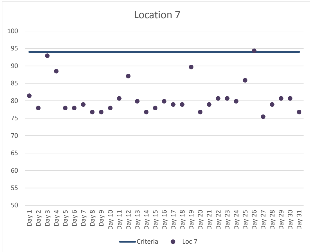
Figure 8. Location 7 Maximum Daily Construction Vibration Monitoring Data (VdB) – May 2017
