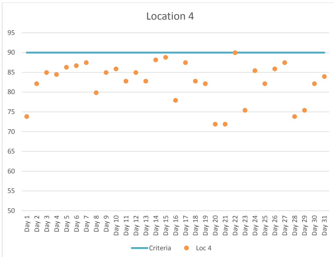
Figure 5. Location 4 Maximum Daily Construction Vibration Monitoring Data (VdB) – May 2017
