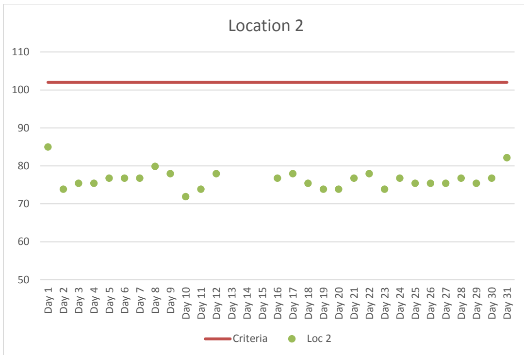
Figure 3. Location 2 Maximum Daily Construction Vibration Monitoring Data (VdB) – May 2017
