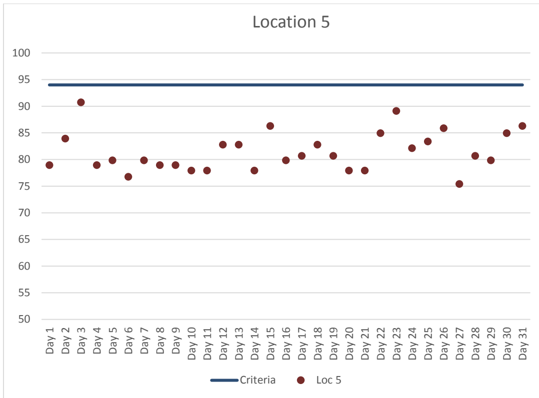
Figure 6. Location 5 Maximum Daily Construction Vibration Monitoring Data (VdB) – May 2017
