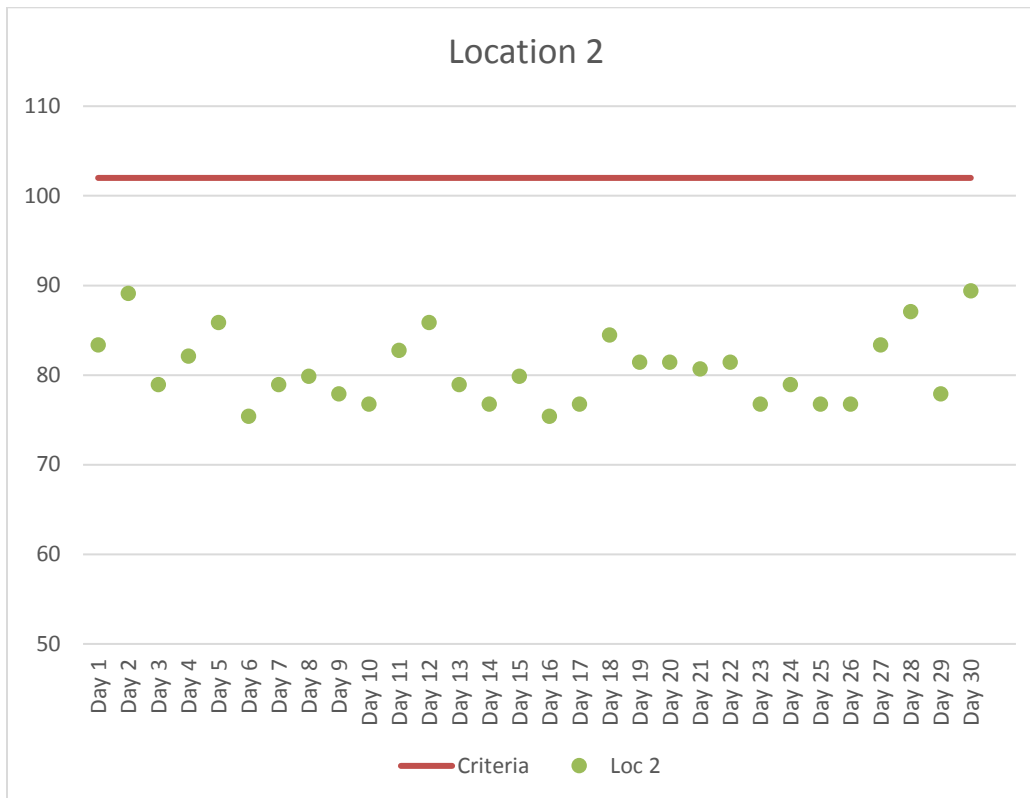
Figure 3. Location 2 Maximum Daily Construction Vibration Monitoring Data (VdB) – December 2017
