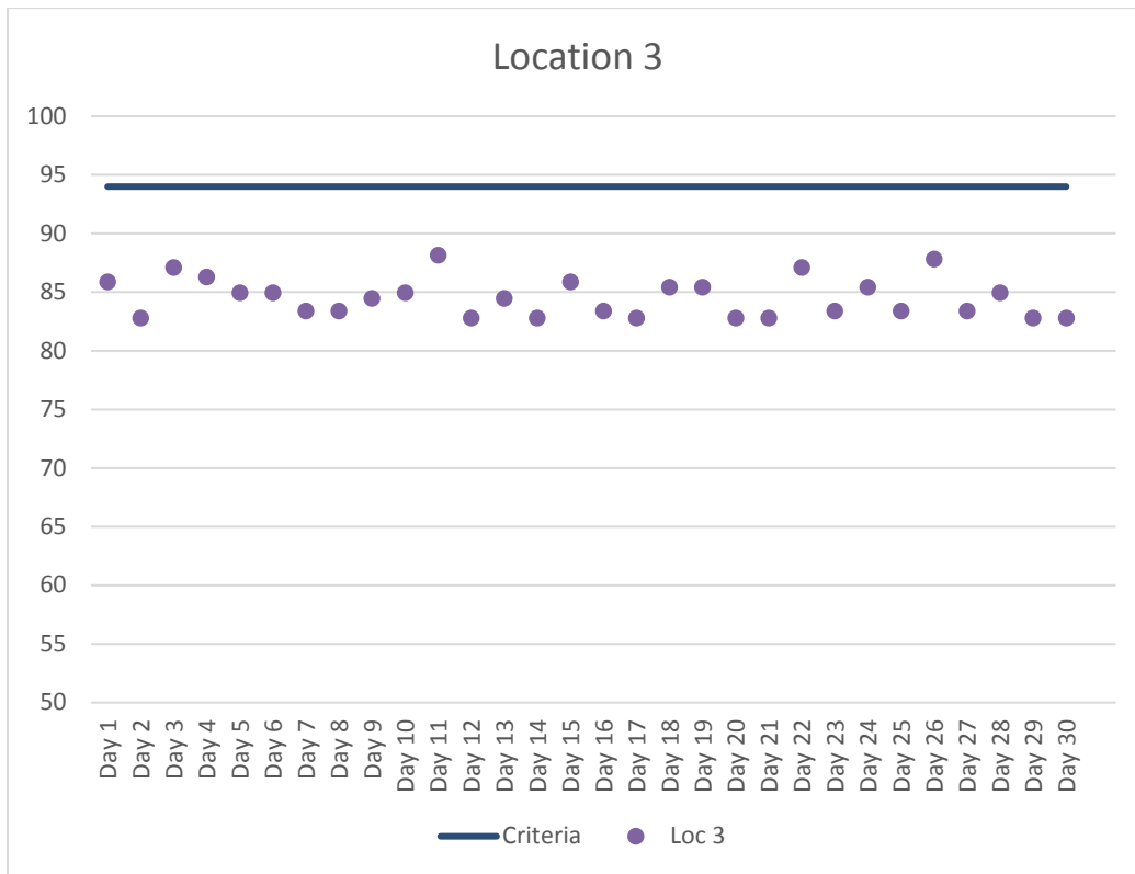
Figure 4. Location 3 Maximum Daily Construction Vibration Monitoring Data (VdB) – December 2017
