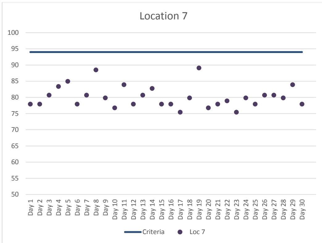
Figure 8. Location 7 Maximum Daily Construction Vibration Monitoring Data (VdB) – December 2017
