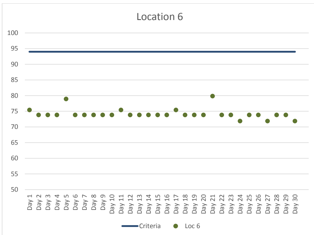
Figure 7. Location 6 Maximum Daily Construction Vibration Monitoring Data (VdB) – December 2017
