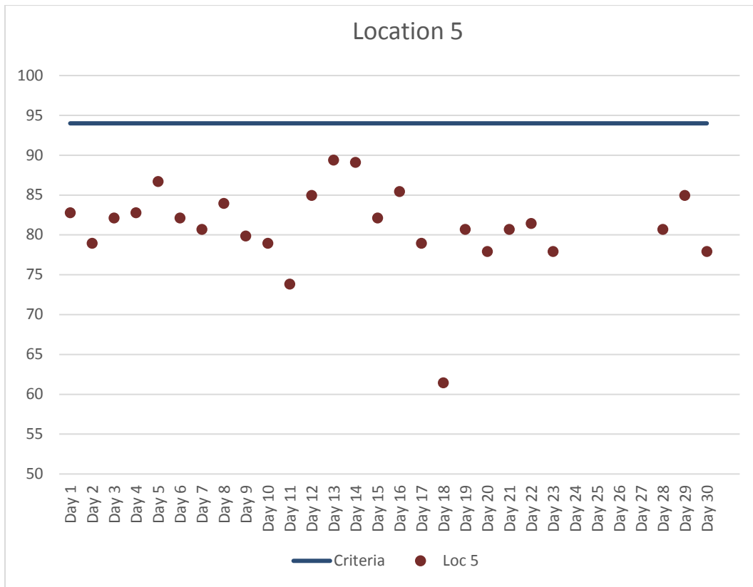
Figure 6. Location 5 Maximum Daily Construction Vibration Monitoring Data (VdB) – December 2017
