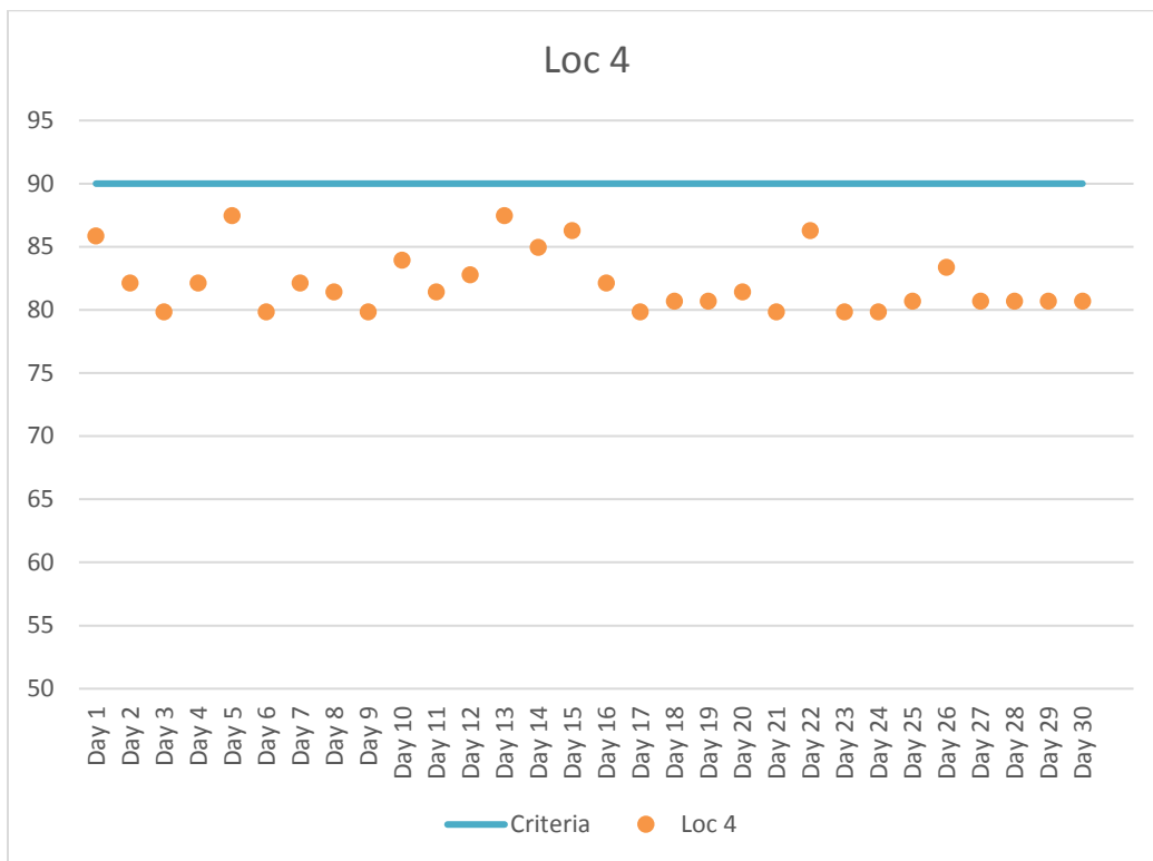
Figure 5. Location 4 Maximum Daily Construction Vibration Monitoring Data (VdB) – December 2017
