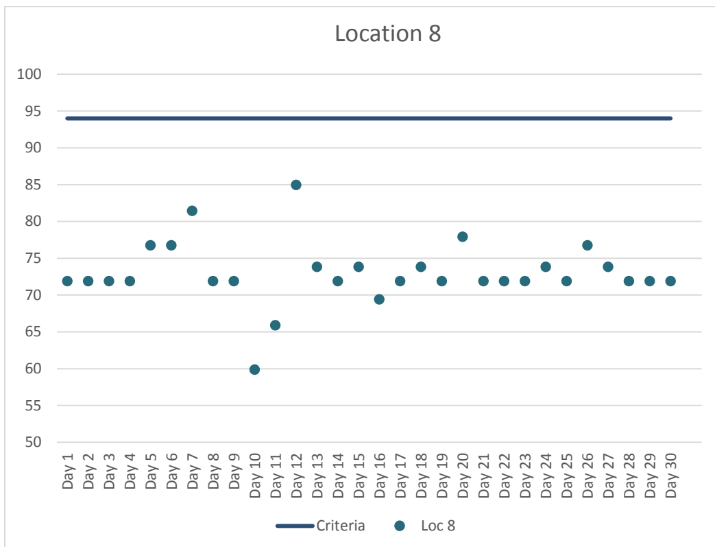
Figure 9. Location 8 Maximum Daily Construction Vibration Monitoring Data (VdB) – December 2017
