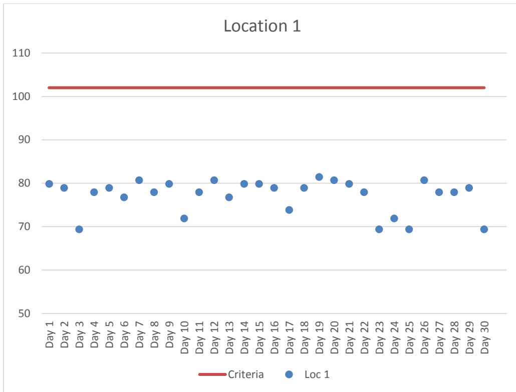
Figure 2. Location 1 Maximum Daily Construction Vibration Monitoring Data (VdB) – December 2017
