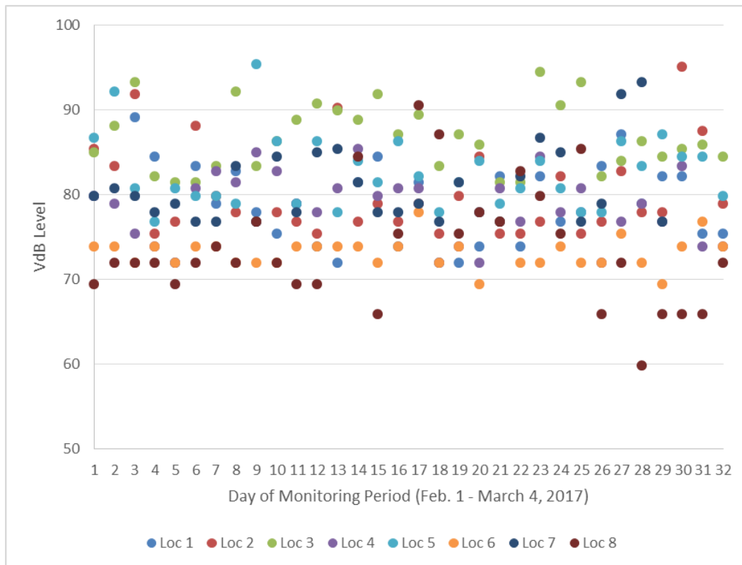
Figure 2. Summary of Maximum Daily Construction Vibration Monitoring Data (VdB) – February 2017
