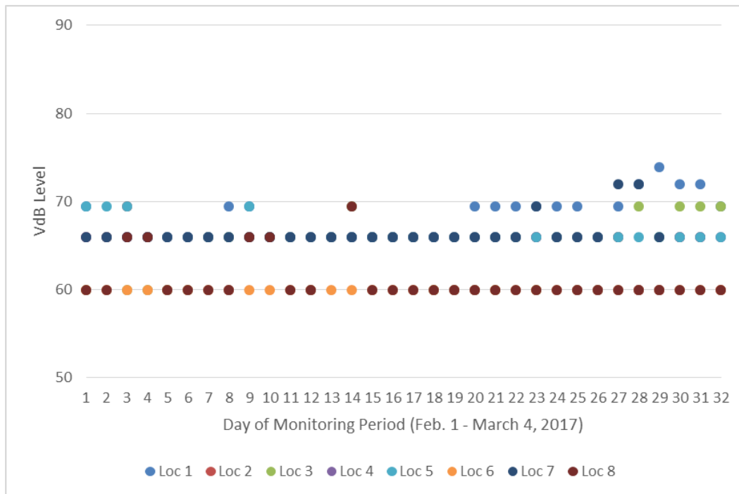
Figure 3. Summary of Average Daily Construction Vibration Monitoring Data (VdB) – February 2017
