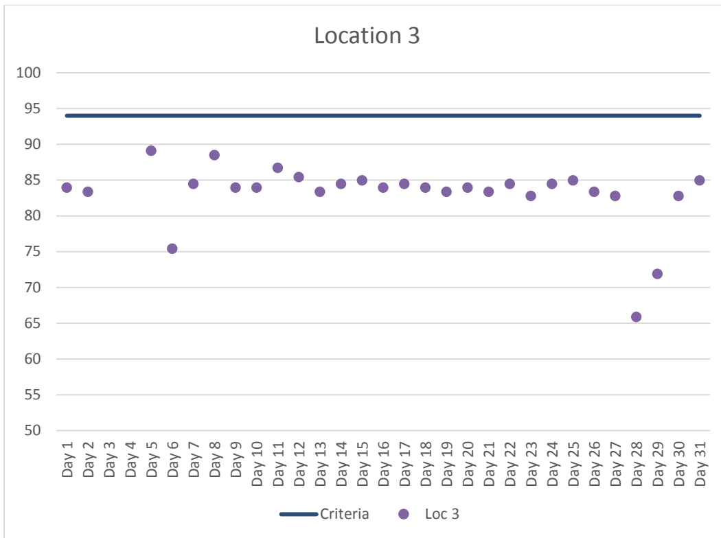
Figure 4. Location 3 Maximum Daily Construction Vibration Monitoring Data (VdB) – July 2017
