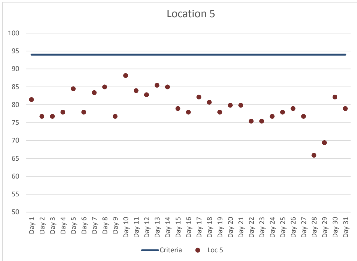
Figure 6. Location 5 Maximum Daily Construction Vibration Monitoring Data (VdB) – July 2017
