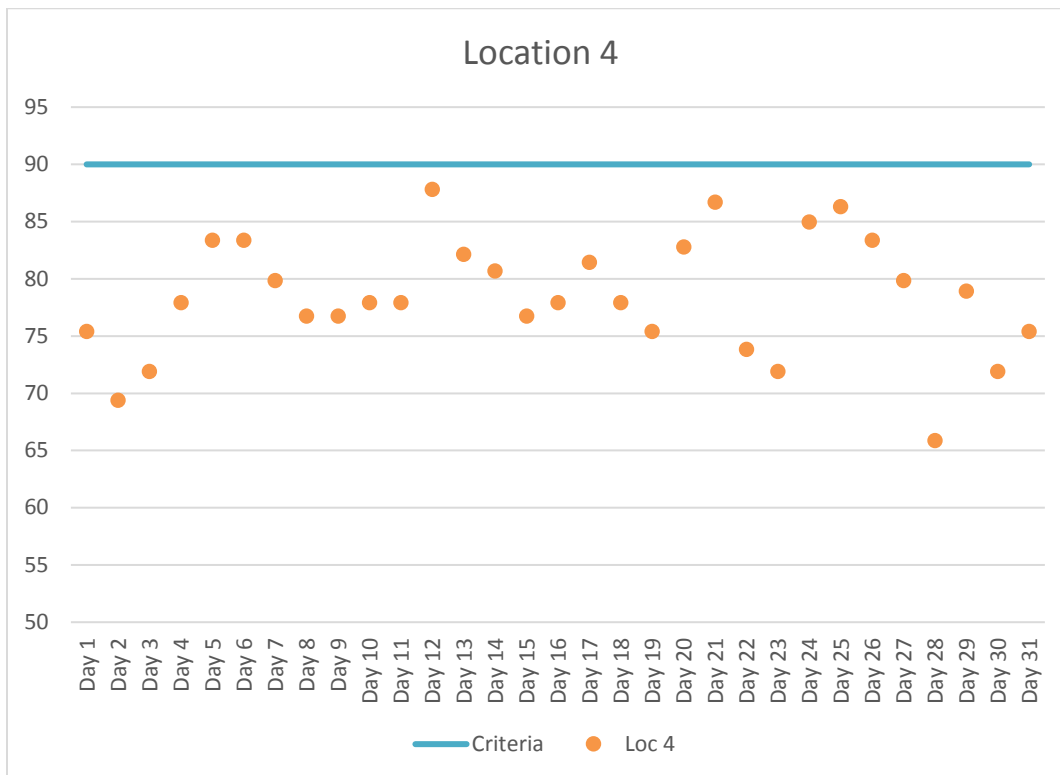
Figure 5. Location 4 Maximum Daily Construction Vibration Monitoring Data (VdB) – July 2017
