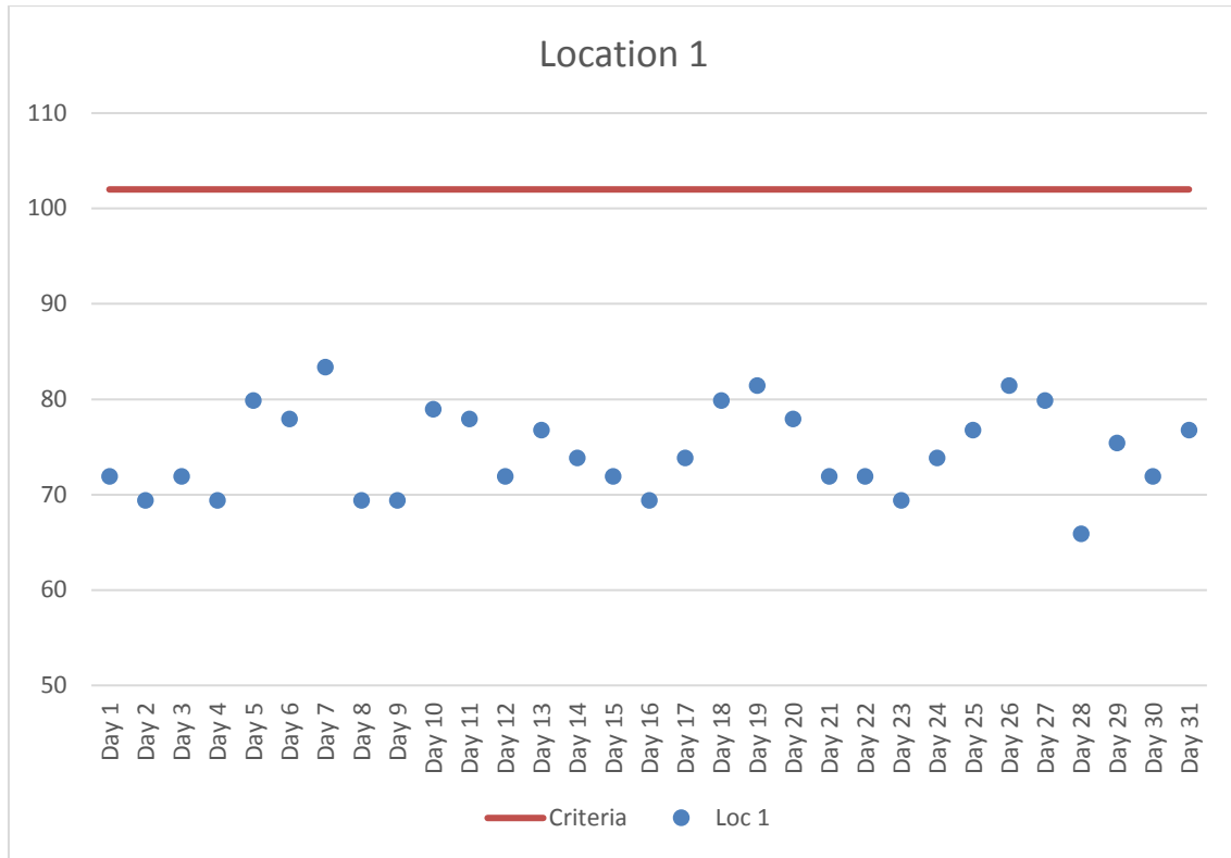
Figure 2. Location 1 Maximum Daily Construction Vibration Monitoring Data (VdB) – July 2017
