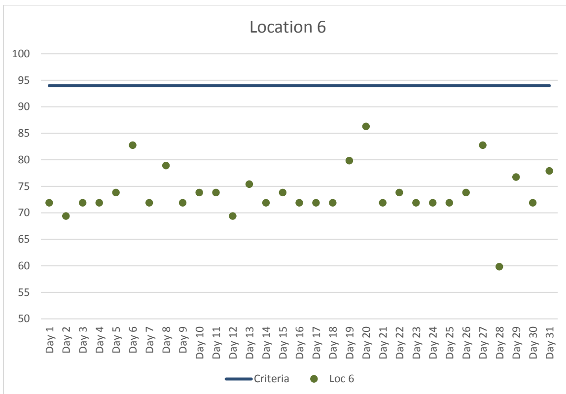
Figure 7. Location 6 Maximum Daily Construction Vibration Monitoring Data (VdB) – July 2017
