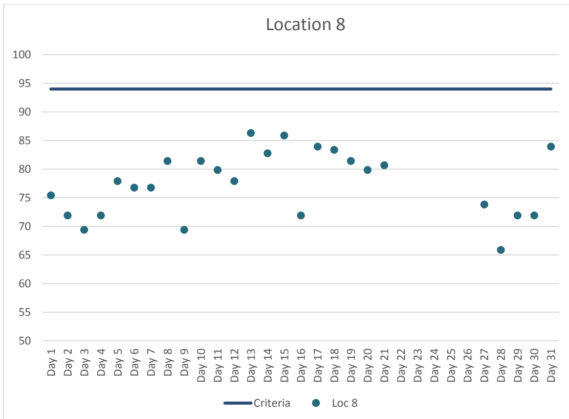
Figure 9. Location 8 Maximum Daily Construction Vibration Monitoring Data (VdB) – July 2017
