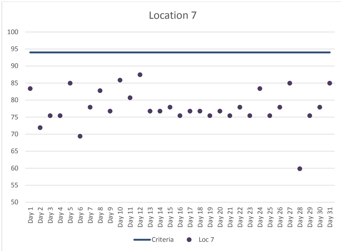
Figure 8. Location 7 Maximum Daily Construction Vibration Monitoring Data (VdB) – July 2017
