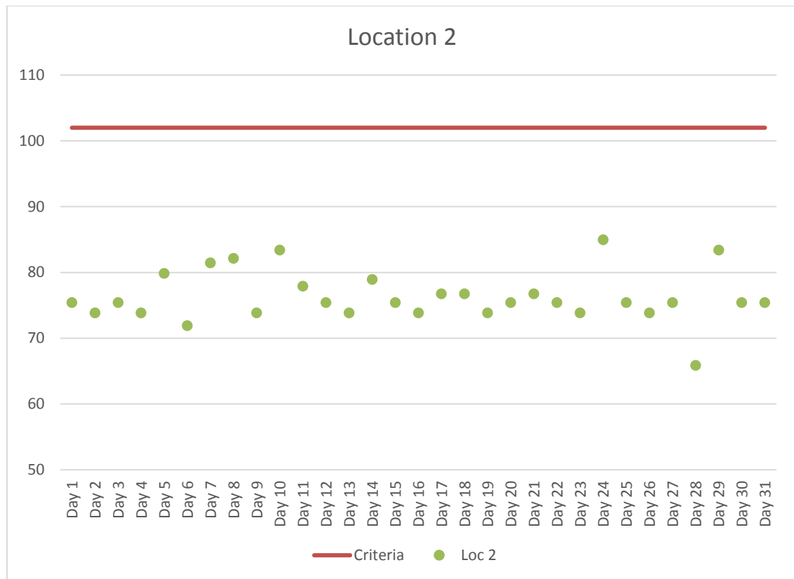
Figure 3. Location 2 Maximum Daily Construction Vibration Monitoring Data (VdB) – July 2017
