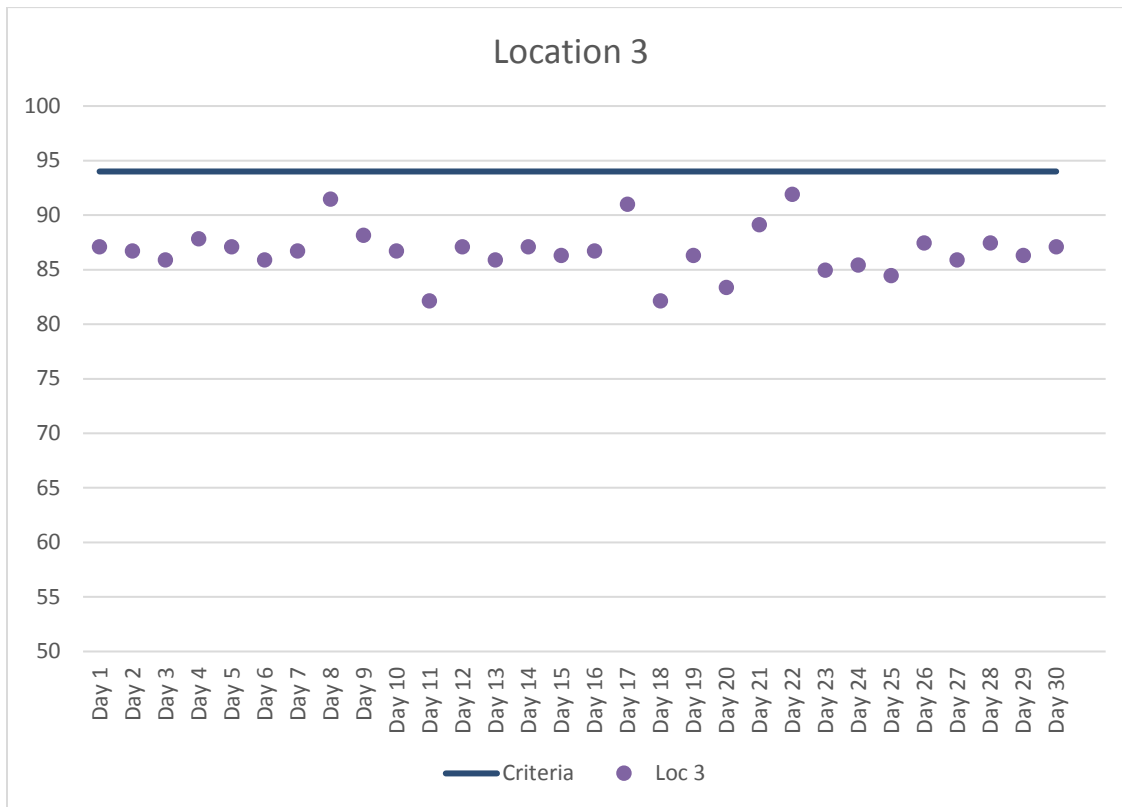
Figure 4. Location 3 Maximum Daily Construction Vibration Monitoring Data (VdB) – November 2017
