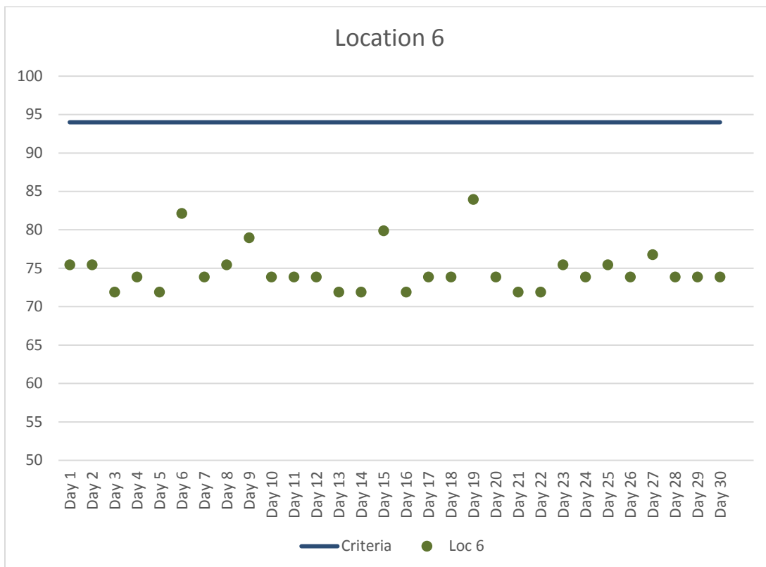
Figure 7. Location 6 Maximum Daily Construction Vibration Monitoring Data (VdB) – November 2017
