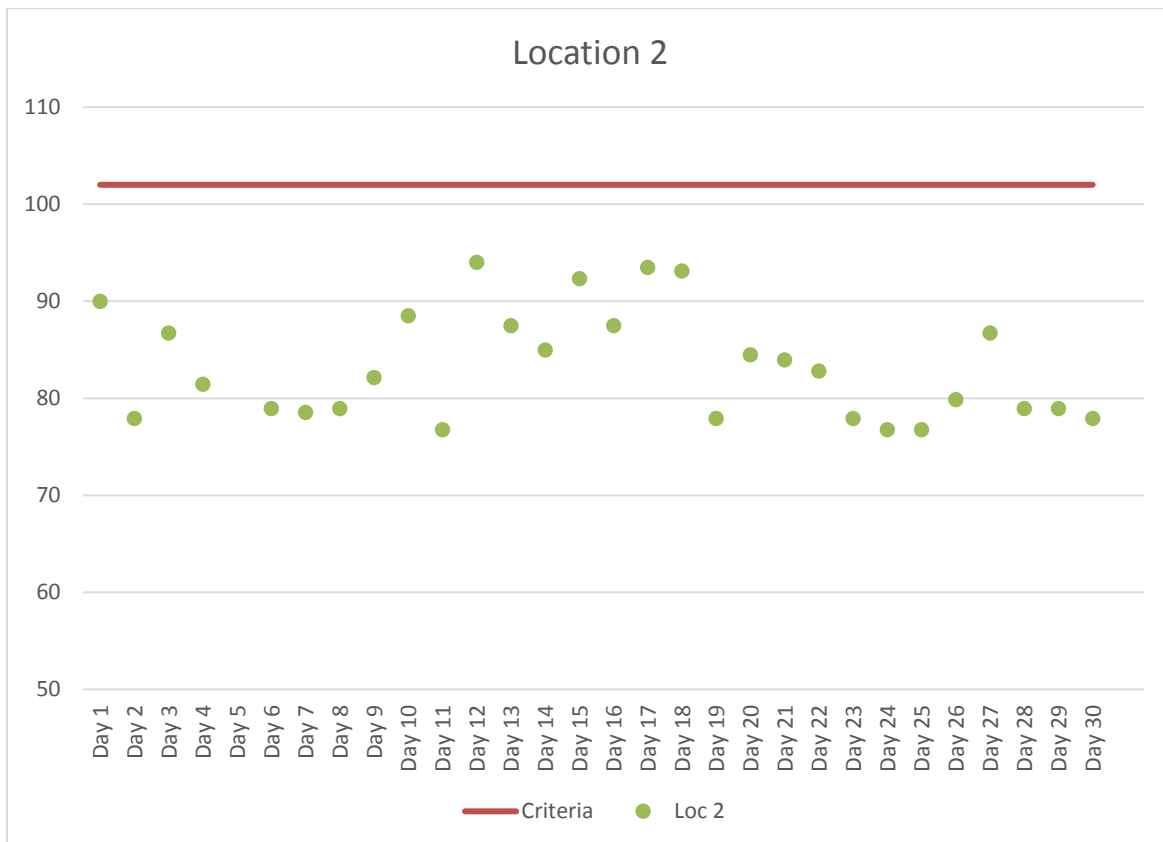
Figure 3. Location 2 Maximum Daily Construction Vibration Monitoring Data (VdB) – November 2017
