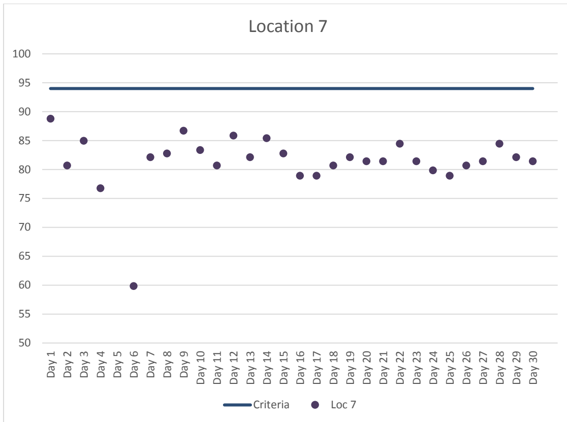
Figure 8. Location 7 Maximum Daily Construction Vibration Monitoring Data (VdB) – November 2017
