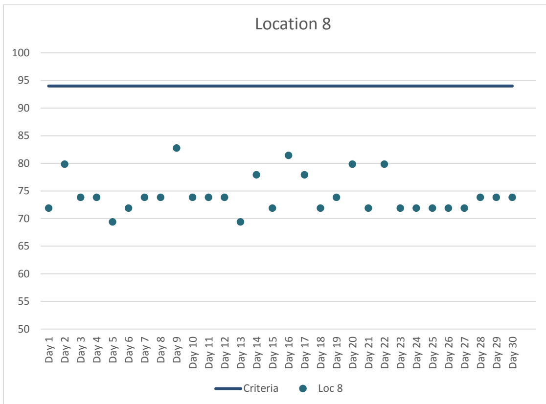
Figure 9. Location 8 Maximum Daily Construction Vibration Monitoring Data (VdB) – November 2017
