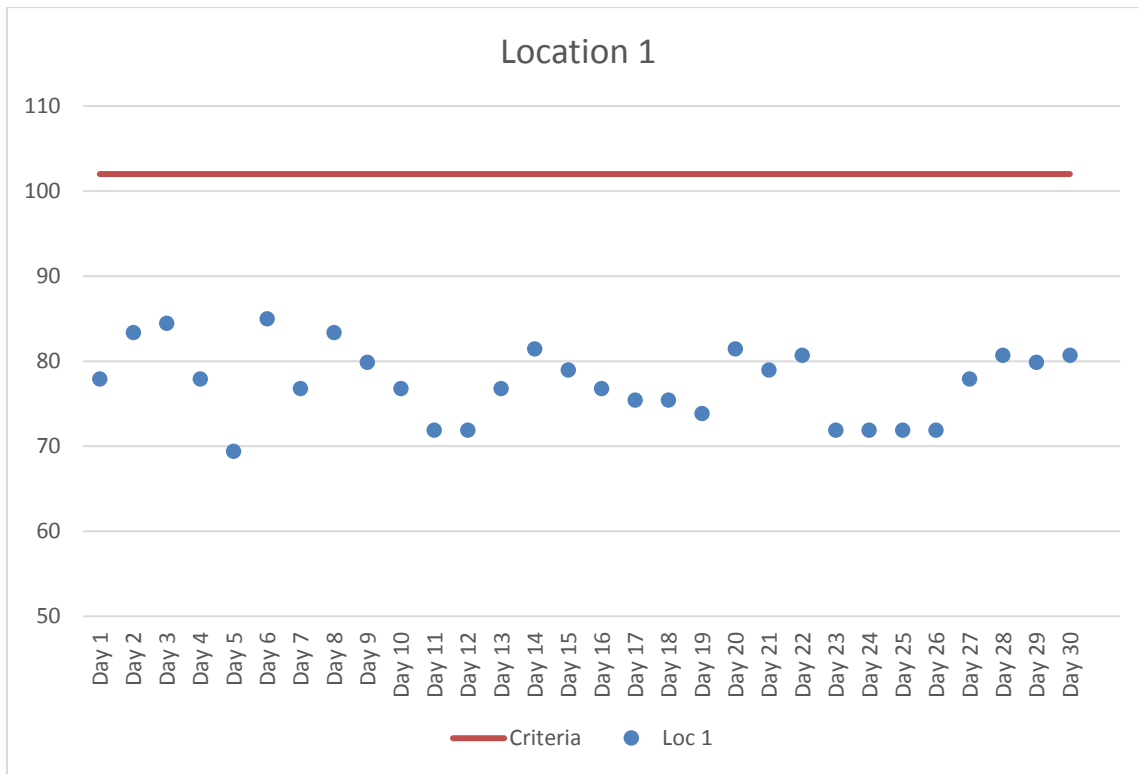
Figure 2. Location 1 Maximum Daily Construction Vibration Monitoring Data (VdB) – November 2017
