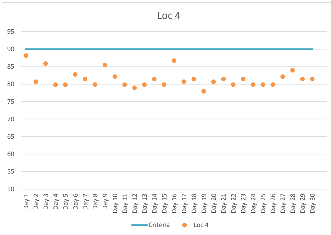
Figure 5. Location 4 Maximum Daily Construction Vibration Monitoring Data (VdB) – November 2017
