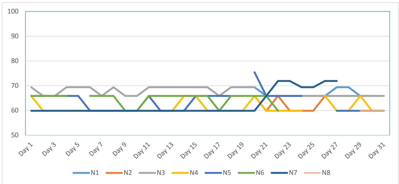
Figure 2. Summary of Construction Vibration Monitoring Data (VdB) – May 2015
